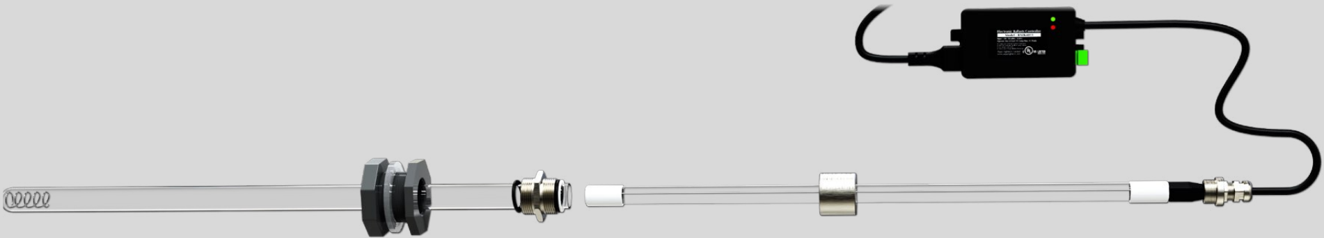
Exploded View
